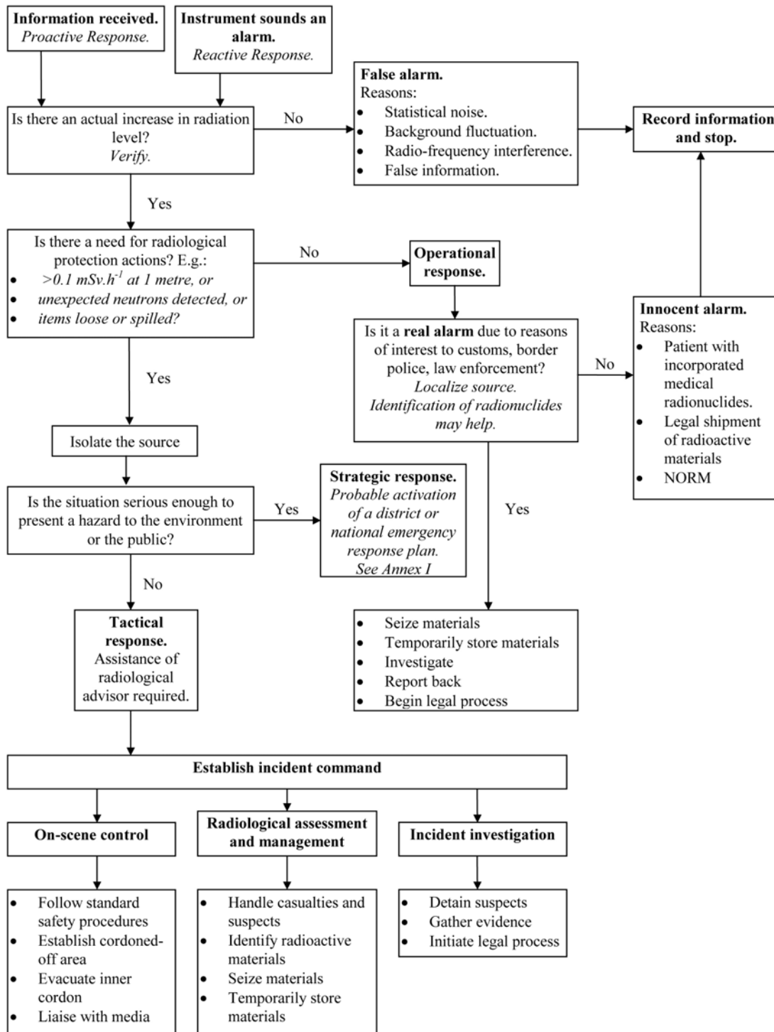
FIG. 1: Flowchart showing the initial response to inadvertent movement or illicit trafficking of radioactive materials. (Reprinted by permission of IAEA, from TECDOC-1313, "Response To Events Involving The Inadvertent Movement Or Illicit Trafficking Of Radioactive Materials.")
